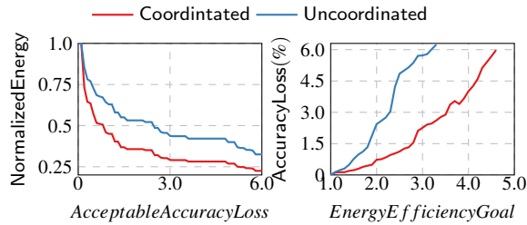
Figure 2: Coordinating application and system provides lower energy for the same acceptable accuracy (left) and lower accuracy loss for the same energy target (right).
