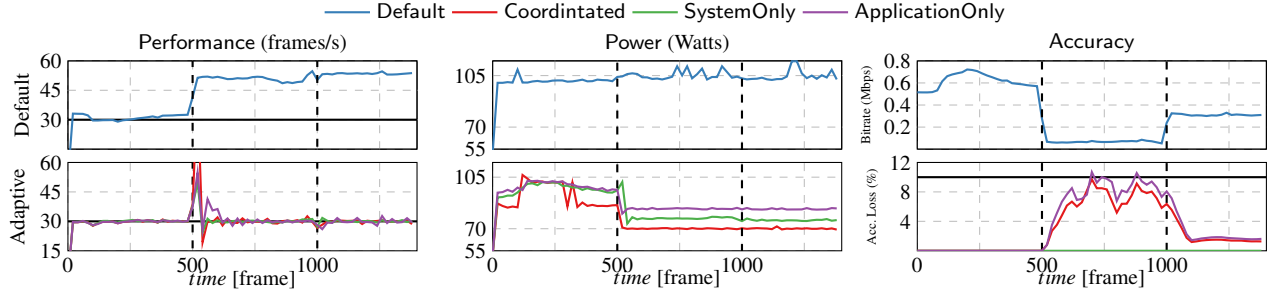
Figure 3: Comparison of non-adaptive behavior and several adaptive schemes adjusting to phases in x264.
