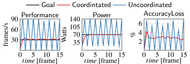
Figure 1: Running an adaptive video encoder on an adaptive system with and without coordination. The goal is to maintain 30 frames per second performance. Without coordination, the performance goal is not met while power and accuracy fluctuate wildly. In contrast, the coordinated approach meets the performance goal while conserving power and accuracy.
