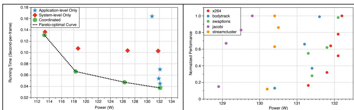
Figure 1: Power and performance tradeoff space for various adaptive techniques on Intel Xeon E5 multicore server when running x264 ( left ). Proposed coordinated management extends the Pareto points to a more efficient operating point. Application adaptation has minimal impact on power consumption on all 5 of the applications ( right ).
