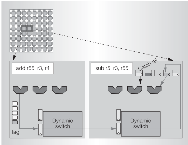
Figure 5. Demultiplexing overview.
